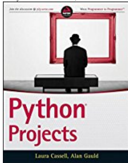
Python Projects
